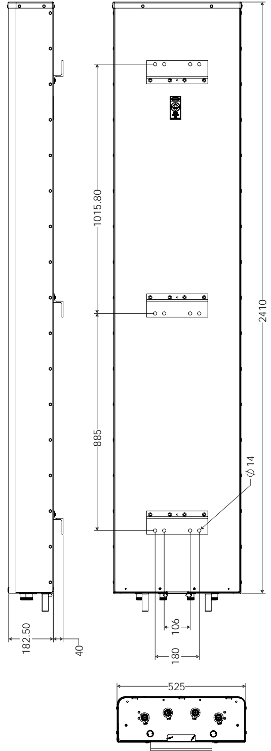
Dimensions (mm)
